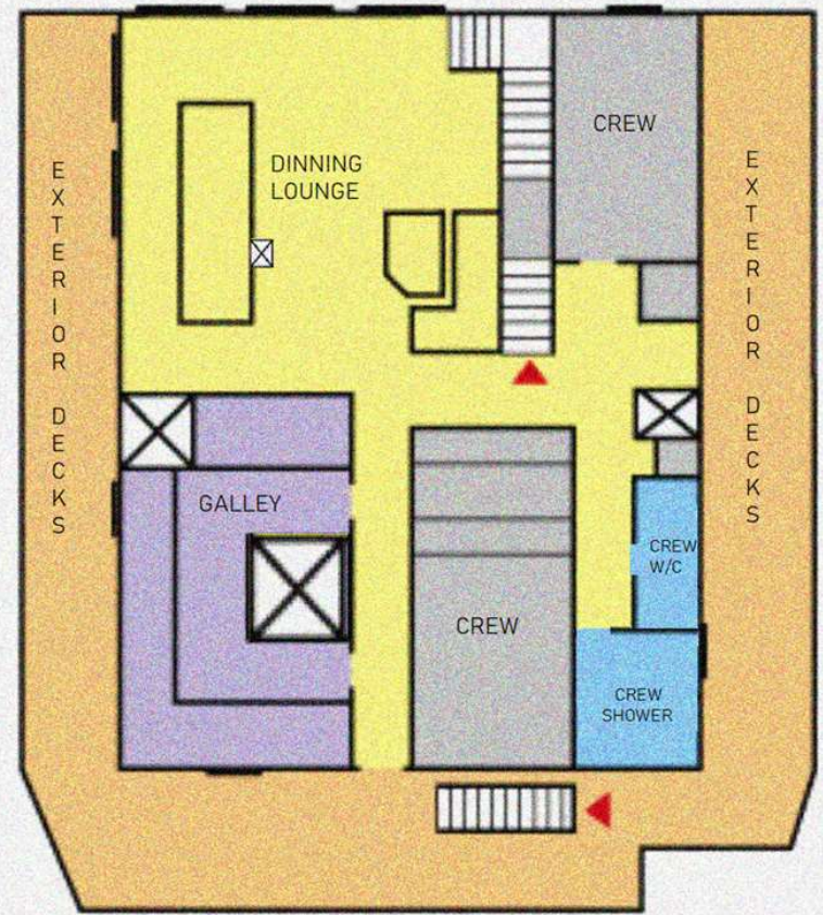
DINNING AND GALLEY DECK
