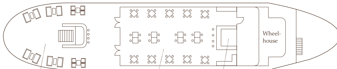
TERRACE DECK
