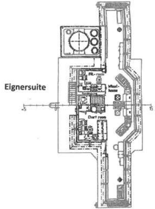
F - Deck
