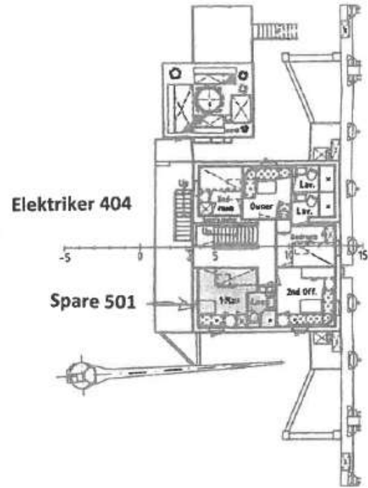
C - Deck
